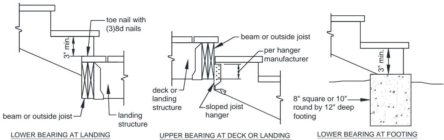
FIGURE 40: STRINGER BEARING
