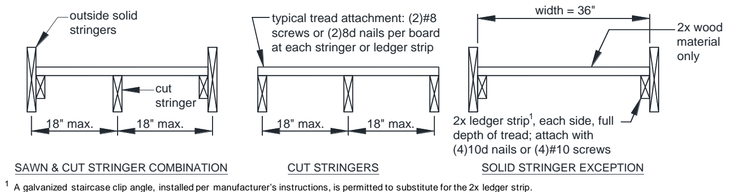
FIGURE 42: STRINGER TREADS
