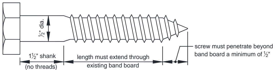
FIGURE 27: LAG SCREW
